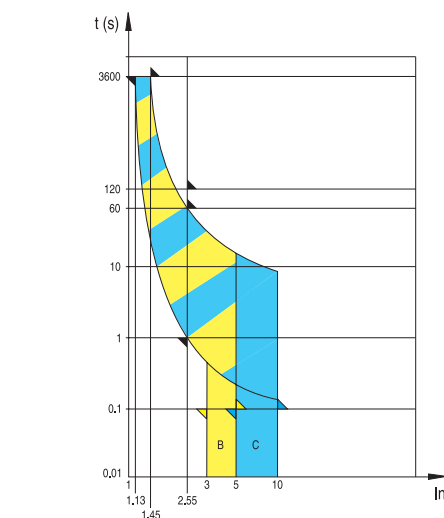
Tripping characteristic curves (EN/IEC 60898-1)
