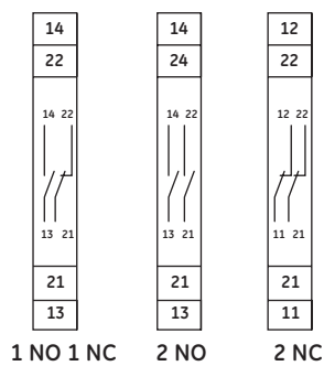
Add-on auxiliary contact
