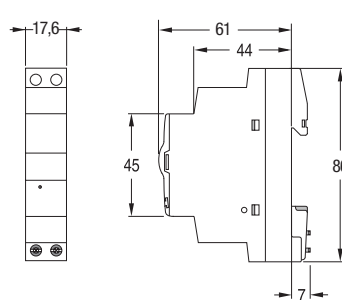
SurgeGuard safety module
