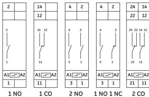
Impulse switches
